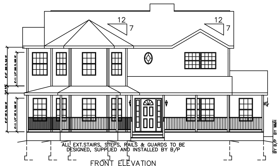
FRONT ELEVATION
